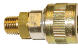
Schrader Style Socket Male Threads
